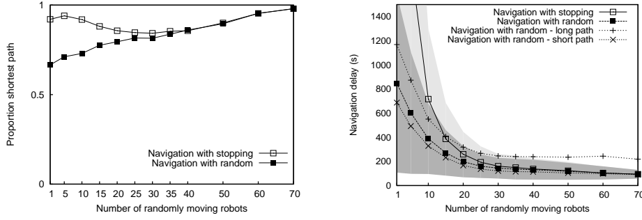
Fig. 9 Test results in the cluttered environment of Figure 8 for a single searching robot and an increasing number of randomly moving robots. For both the NwS and the NwR strategies, we show the fraction of runs in which the searcher uses the short path (left), and the average time needed for navigation (right). Shaded areas around the average navigation delay curves show the standard deviation (compared to other tests, standard deviations are lower here, because searcher and target do not start from random positions; see Section 3.2). For the NwR strategy, we also show the average navigation delay when splitting up the results according to the path taken by the robots.
