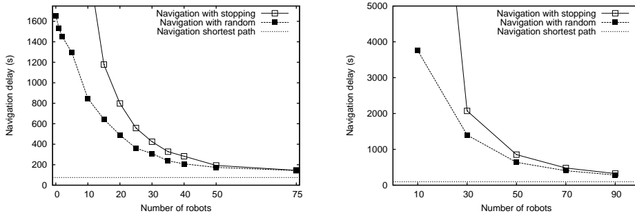
Fig. 7 Test results in the cluttered environments of Figure 6 for a single searching robot and an increasing number of randomly moving robots. The left plot refers to Figure 6 (left), and the right one to Figure 6 (right). In both figures, the results for NwS and NwR are reported together with the performance that would be obtained by following the shortest path.
